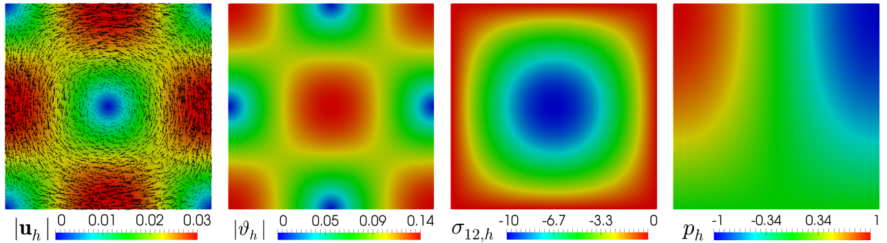
Figure 6.1: [Example 1]: Computed magnitude of the velocity and velocity gradient, viscoelastic pseudostress tensor component, and pressure field.
