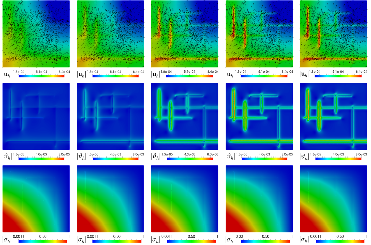
Figure 6.4: [Example 3]: Computed magnitude of the velocity, velocity gradient tensor, and viscoelastic pseudostress tensor at time T = 1 , with \rho = 4 , fracture setting F = 10 and D = 1 , and porous media setting F = 1 and D = 1000 , for \kappa \in \{3, 2, 1, 10^{-2}, 10^{-4}\} (from left to right).
