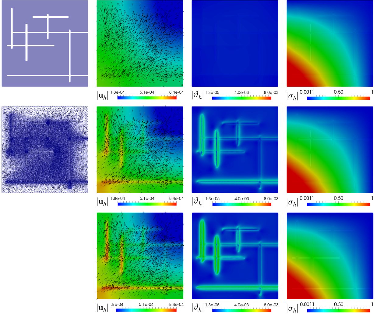
Figure 6.3: [Example 3]: Domain configuration and prescribed mesh (plots in first column), and computed magnitude of the velocity, velocity gradient tensor, and viscoelastic pseudostress tensor at time T = 0.01 (top plots), at time T = 0.5 (middle plots), and at time T = 1 (bottom plots).
