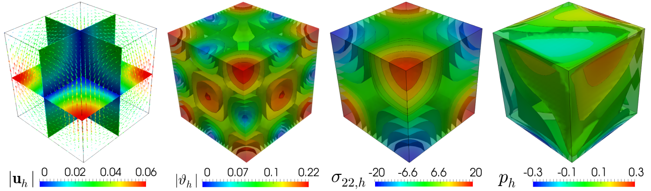
Figure 6.2: [Example 2]: Computed magnitudes of the velocity and velocity gradient, viscoelastic pseudostress tensor component, and pressure field.
